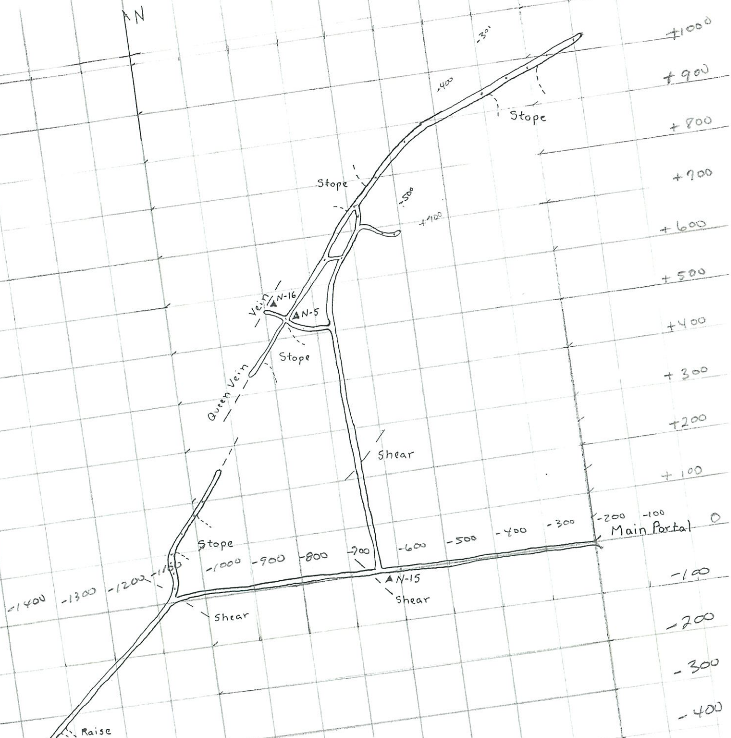
Queen of the Hills Mine 400 Level Mine Plan
